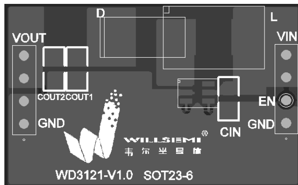
WD3121 Demo Board Layout (Top)
