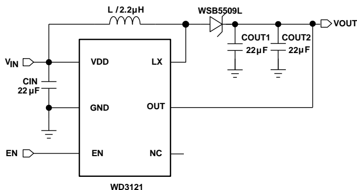
WD3121 Demo Board Schematic
